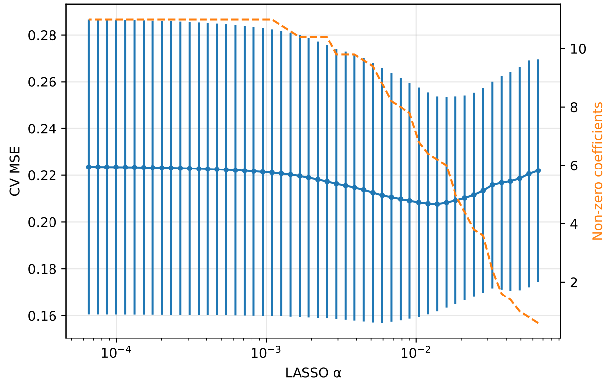
Panel A (N=150, 9 features + Study dummies)
