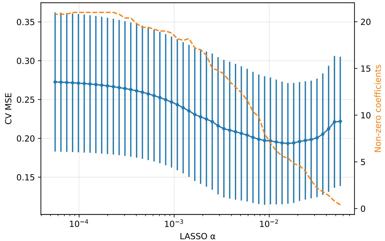
Panel B (N=98, 23 features + Study dummies)
