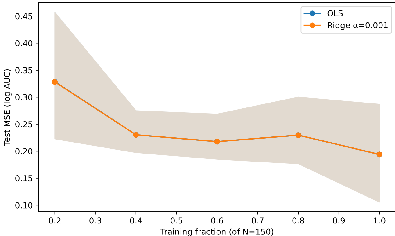
Learning curves — linear baselines (Panel A)
