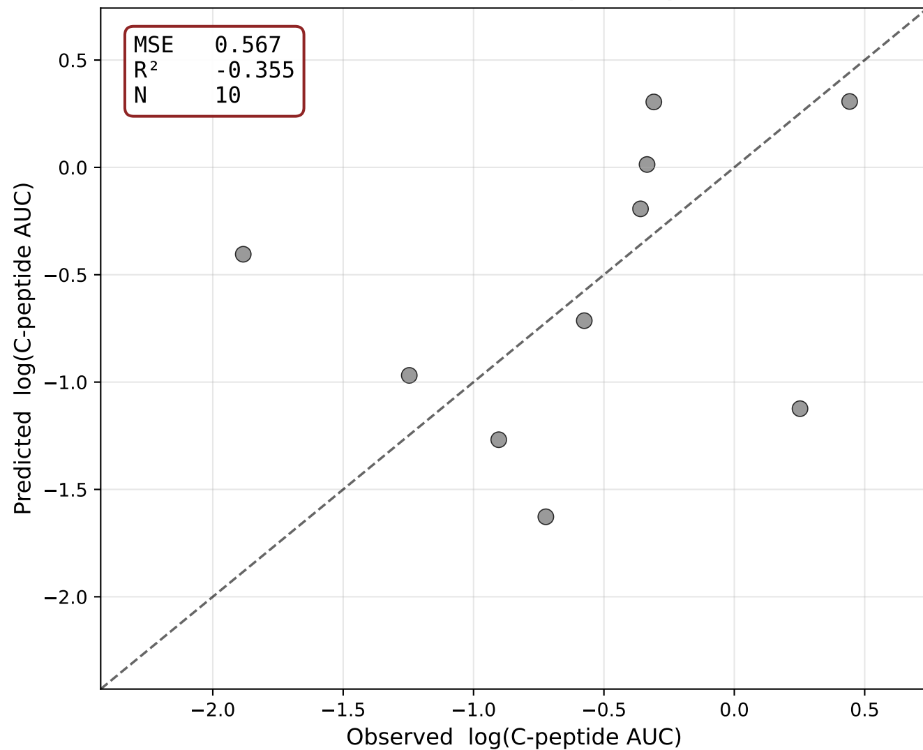
SDY569 alone (N = 10)
