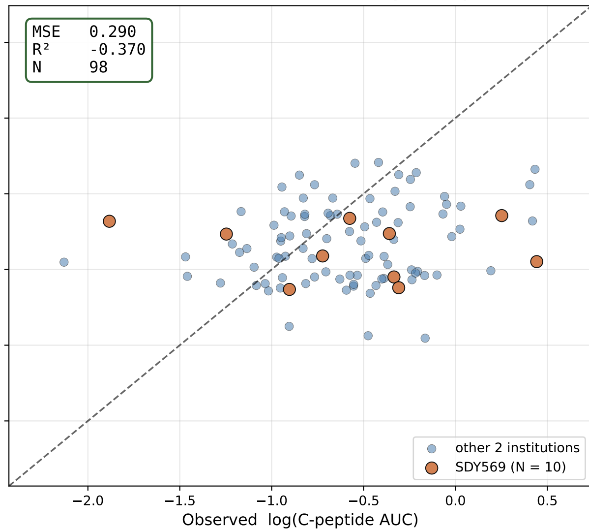
All institutions federated (N = 98)
