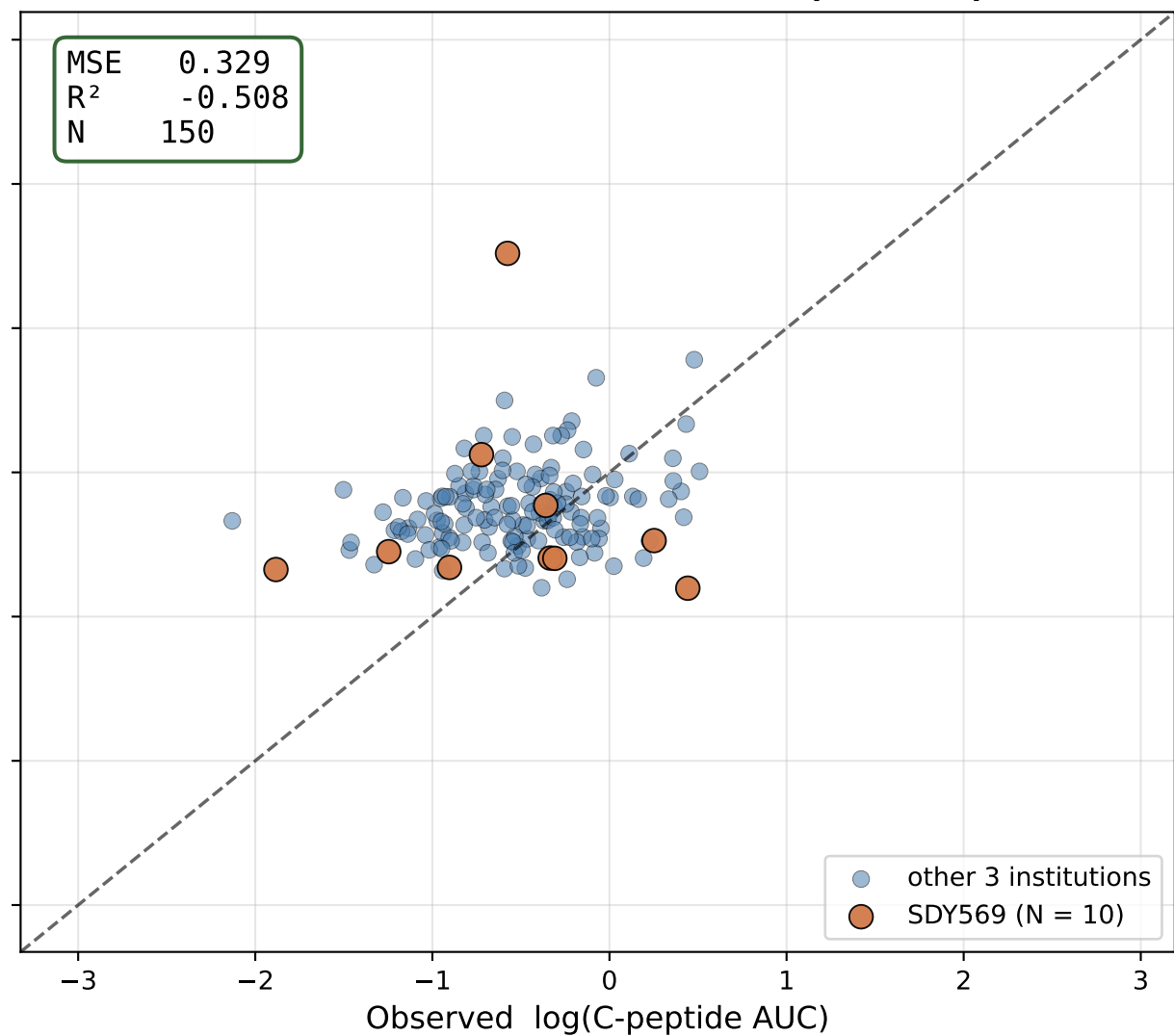
All four institutions federated (N = 150)
