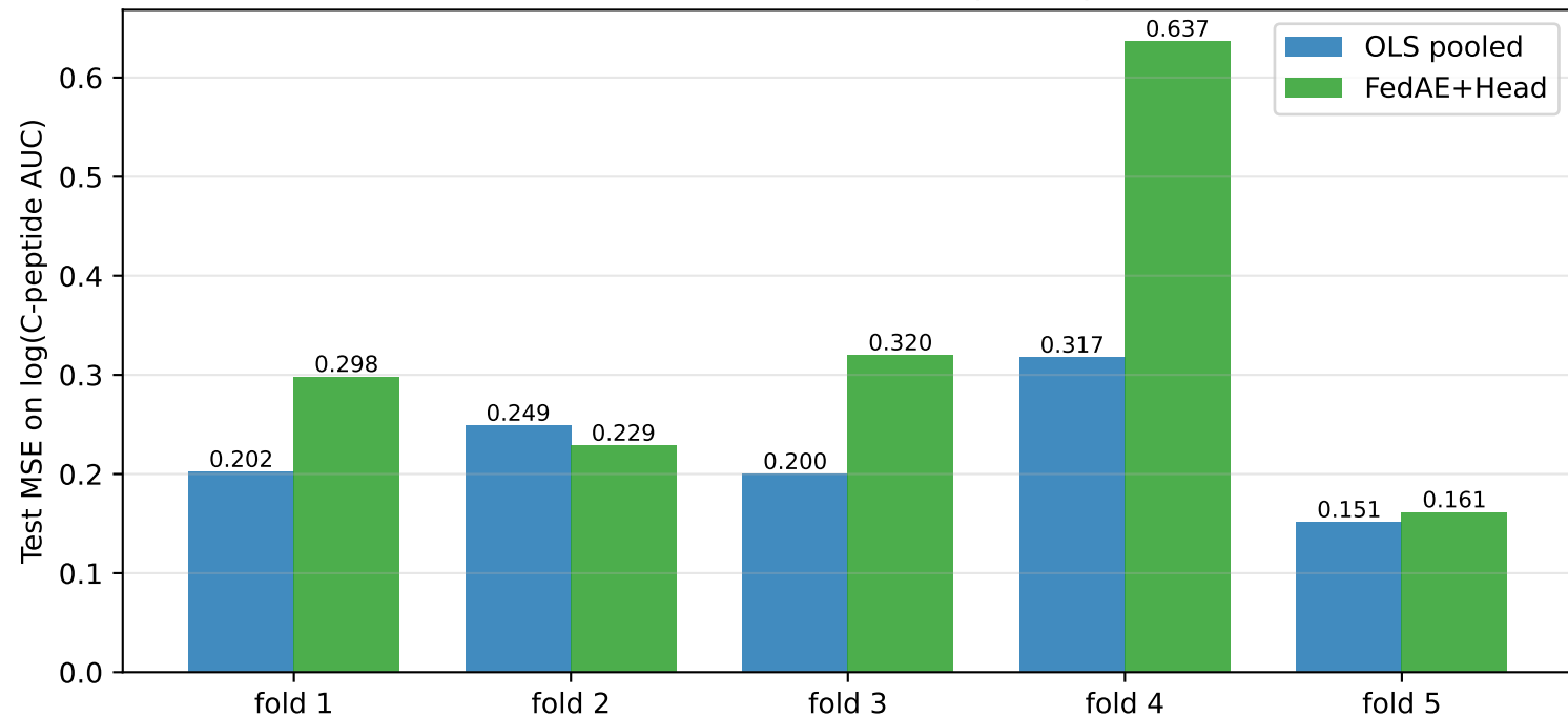
Per-fold MSE: pooled OLS vs Federated AE + frozen-encoder head Panel A, 5-fold stratified-by-Study CV
