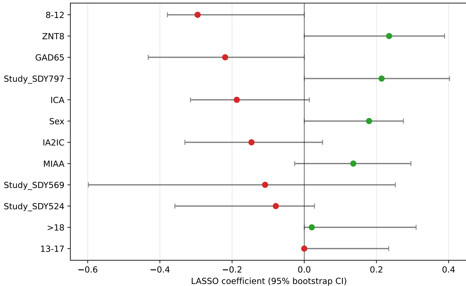
Pooled LASSO coefficients — Panel A
