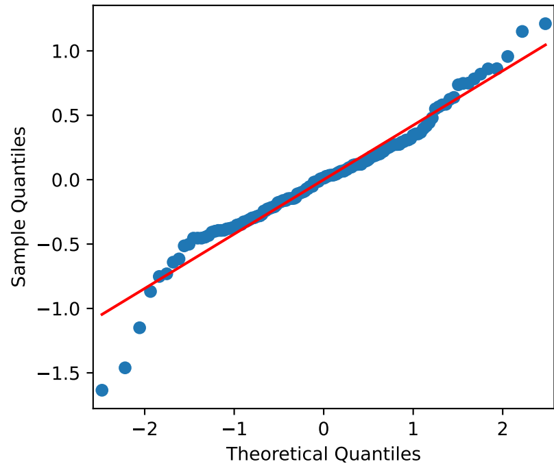
Q-Q plot of residuals
