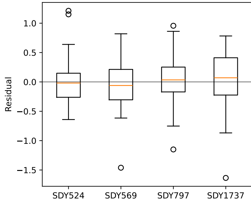
Residuals by Study
