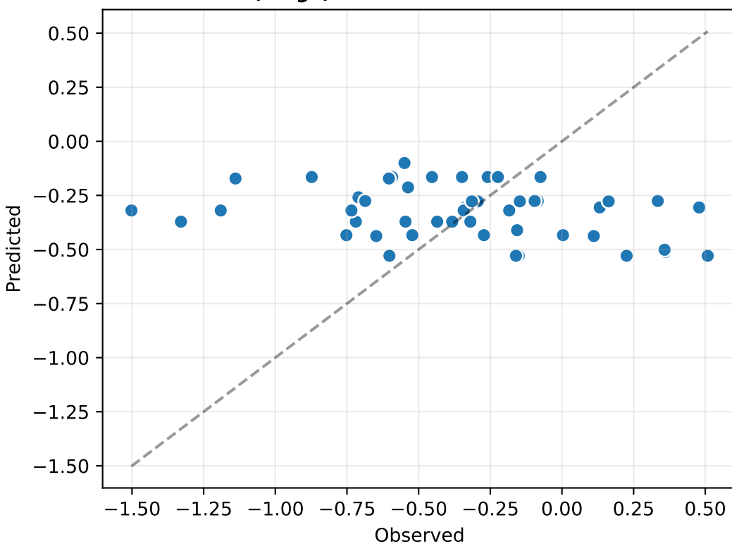
LASSO — SDY797 alone R2 = -0.21
