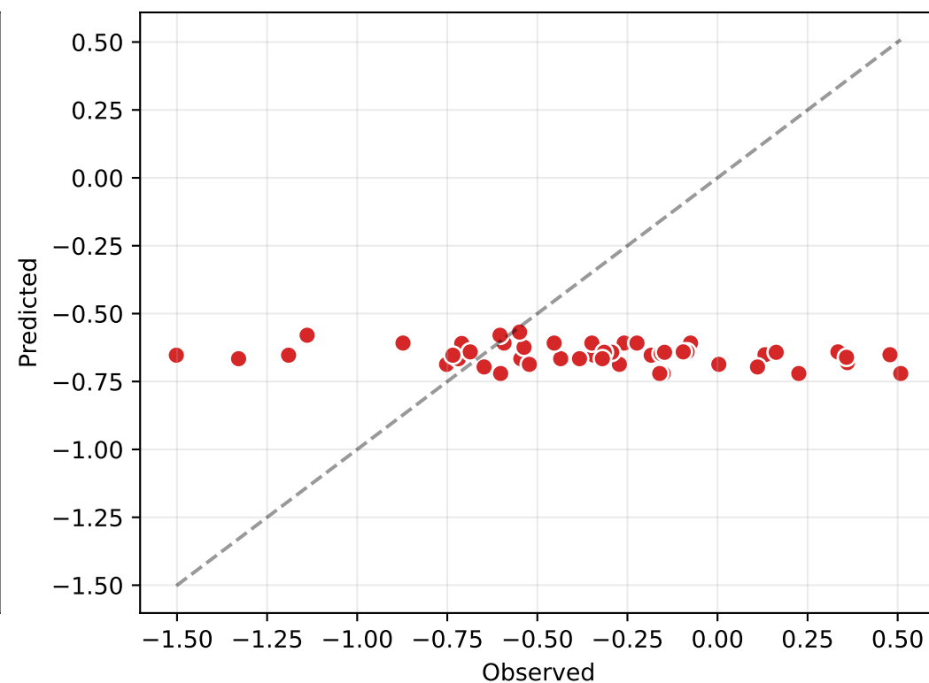
Random Forest — SDY797 + SDY524+SDY569 R2 = -0.07
