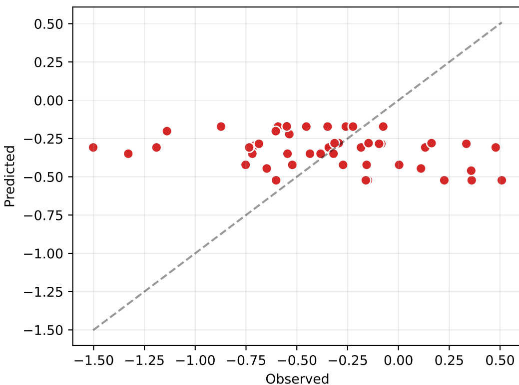
Random Forest — SDY797 alone R2 = -0.22
