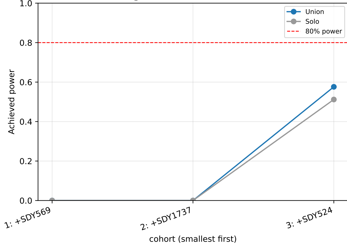
Power grows with cohort — Panel B
