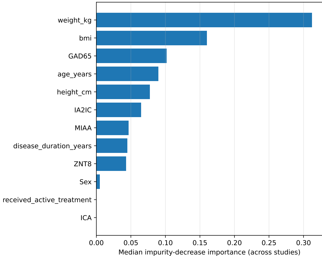
Federated RF importance — Panel B
