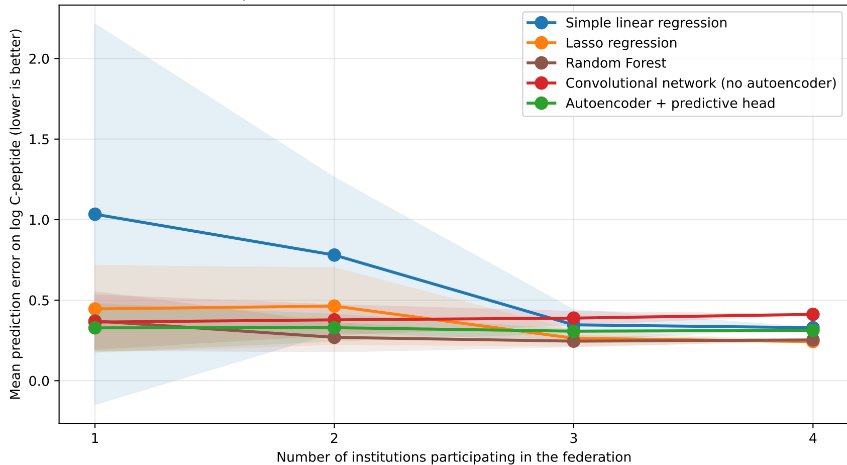
Federation across more institutions improves prediction (panel A: 4 studies, 9 features, 5-fold cross-validation)
