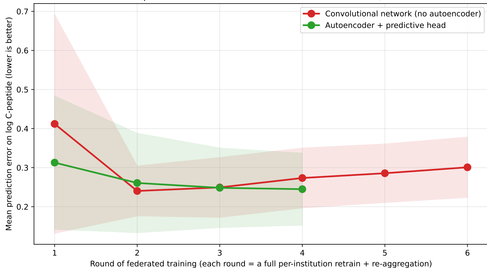
Multi-round federation extracts further benefit from the same data (panel A, all four institutions, 5-fold cross-validation)
