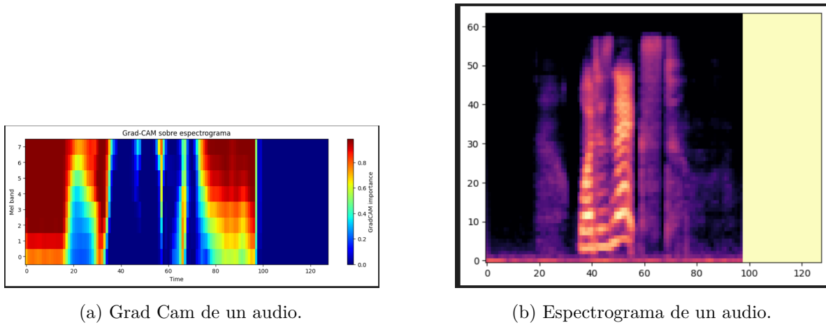
Figura 3.14: Grad Cam local espectrogramas Wav2Vec2
