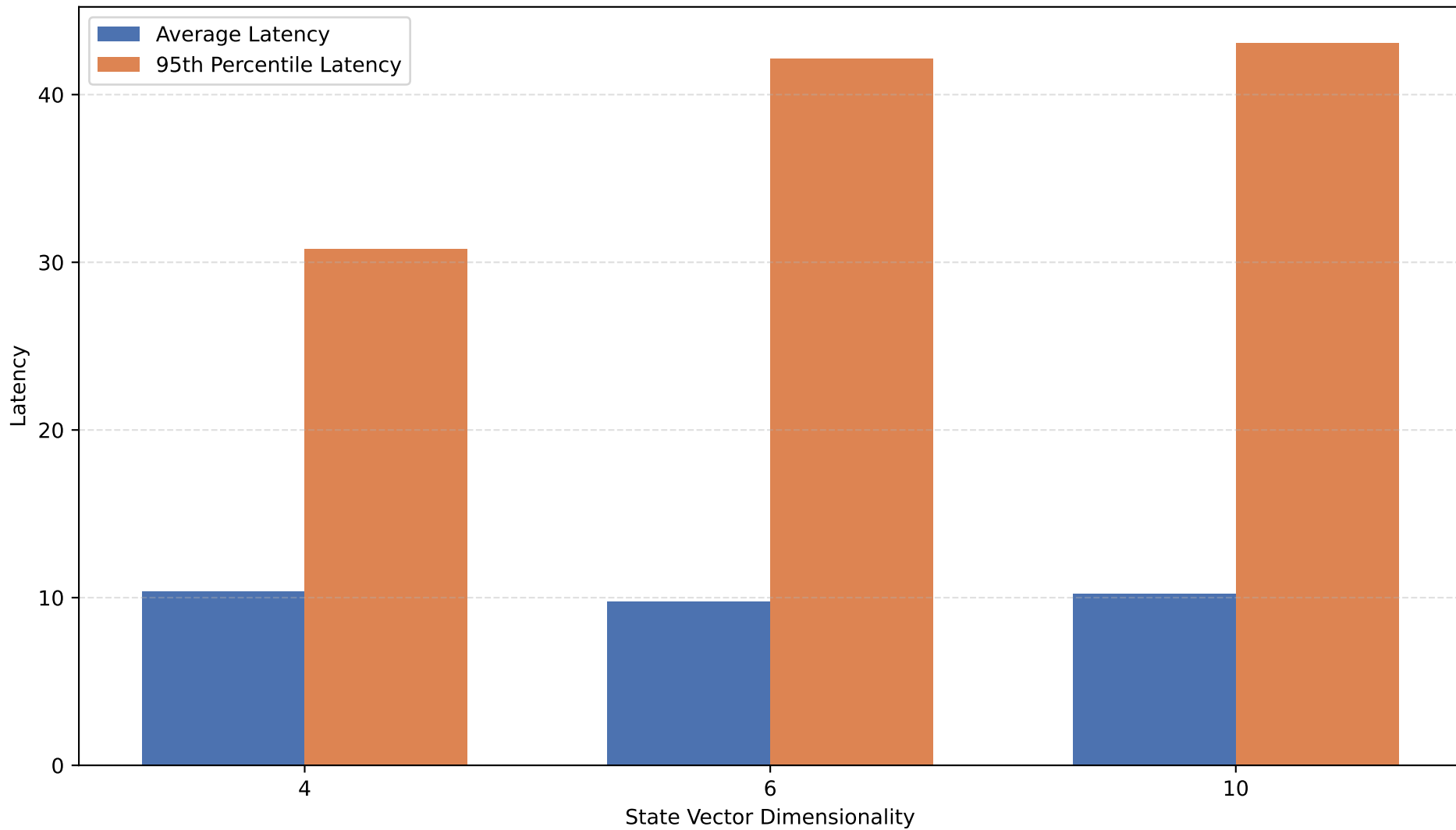
Latency Metrics vs State Dimensionality
