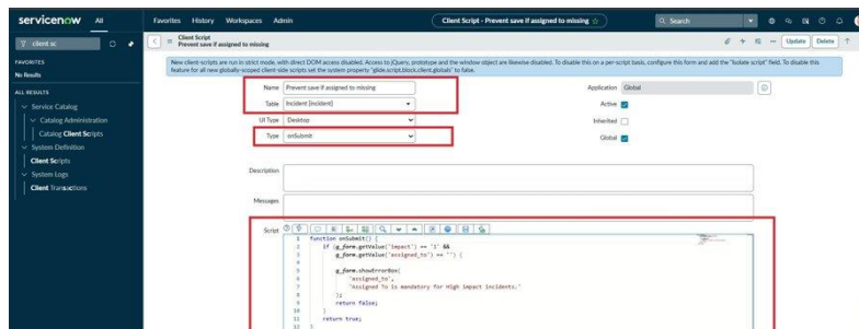
Fig 7: onSubmit client script
