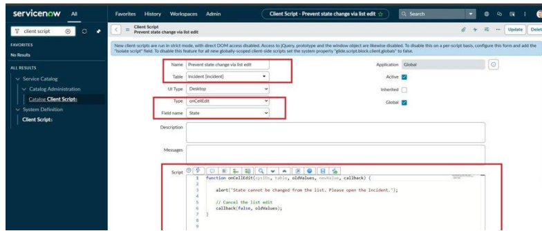
Fig 8: onCellEdit client script
