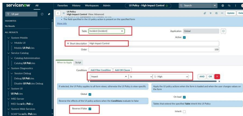
Fig 2: High Impact Control UI Policy
