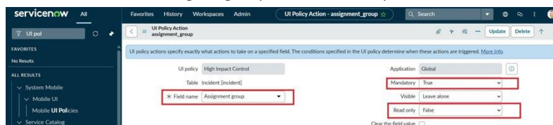
Fig 3: UI Policy Action: Assignment group
