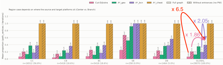
Algorithm performance by graph region: full graph vs graph without entrances
