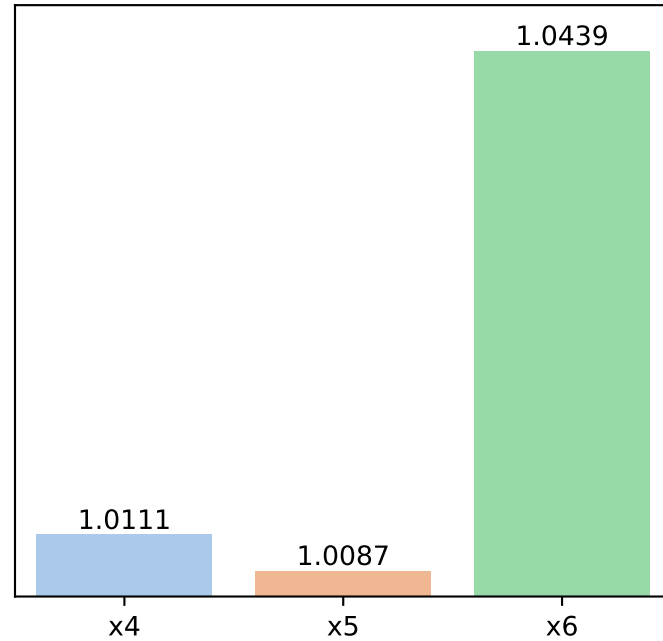
RMSE
