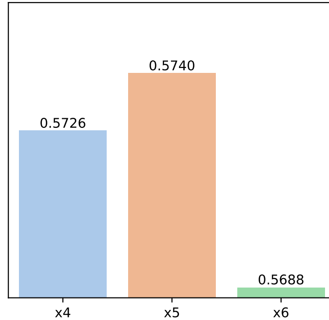
NDCG
