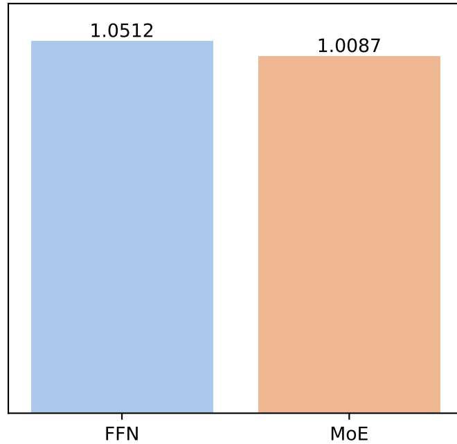
RMSE
