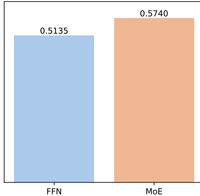
NDCG
