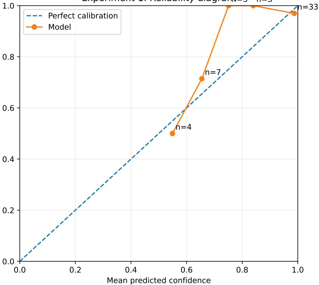
Experiment 1: Reliability diagram
