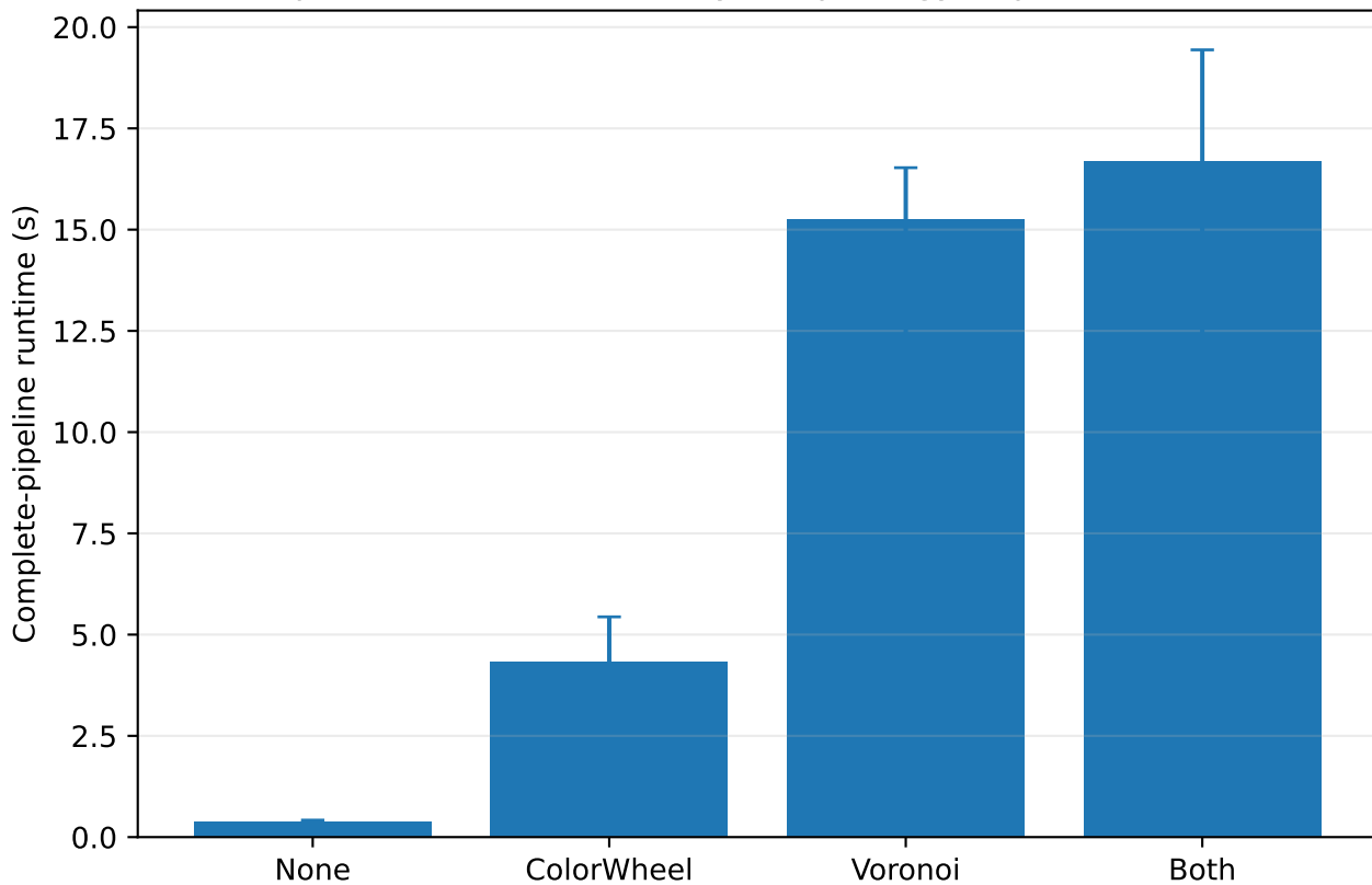
Experiment 3C: Runtime by morphology-dependent route
