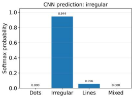
CNN class probabilities
