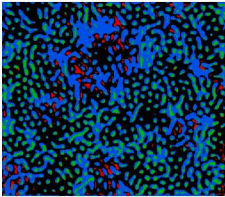
Segmentation disagreement
