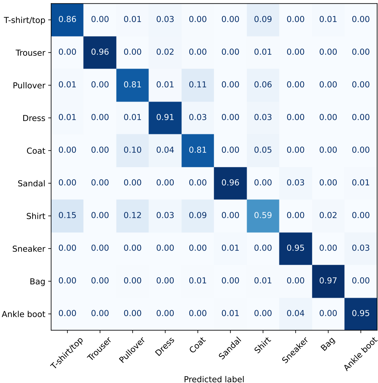
Random forest: confusion matrix (test set)
