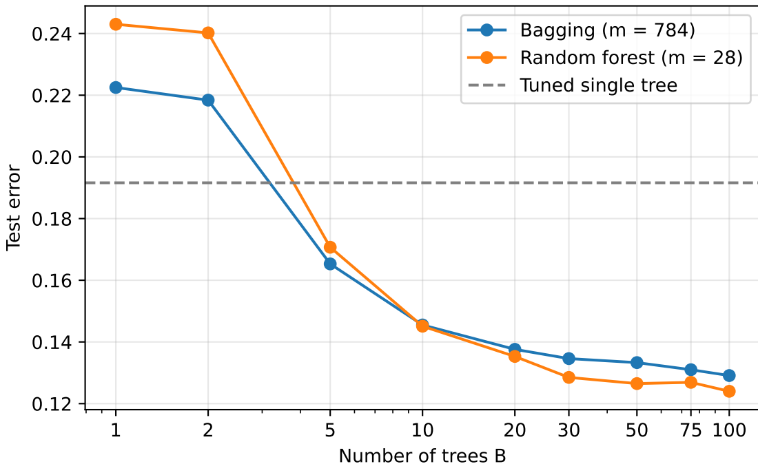
Test error vs. number of trees
