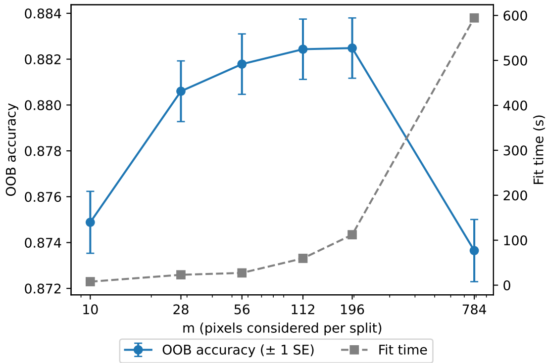
Random forest: choice of m ( B = 100 )
