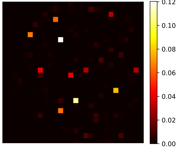
Decision tree (tuned) 50% of importance in 6 pixels
