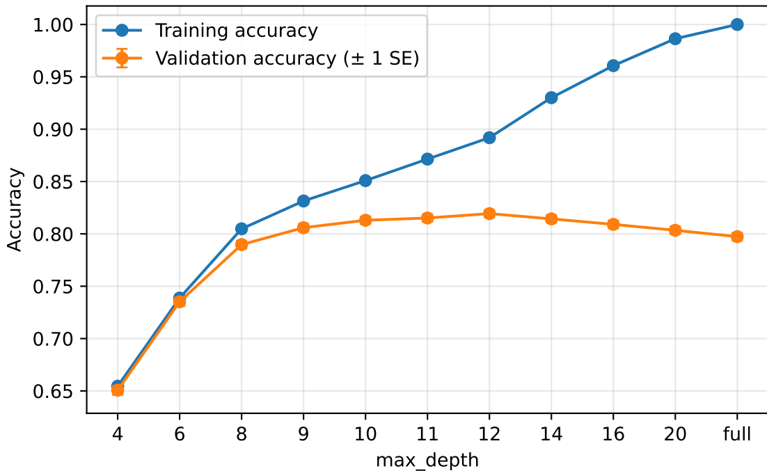
Decision tree: training vs validation accuracy
