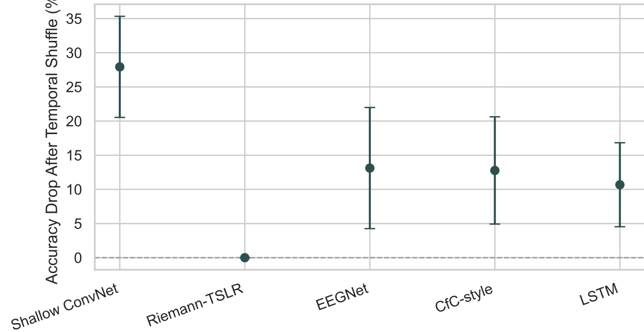
Session-wise Temporal Shuffle Control
