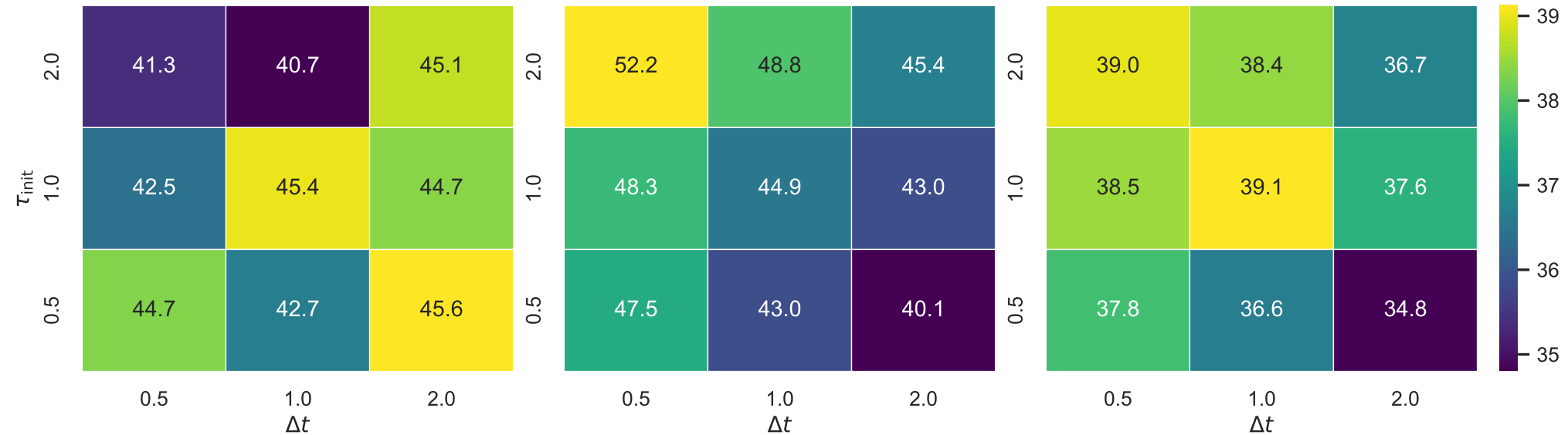
CfC-style
