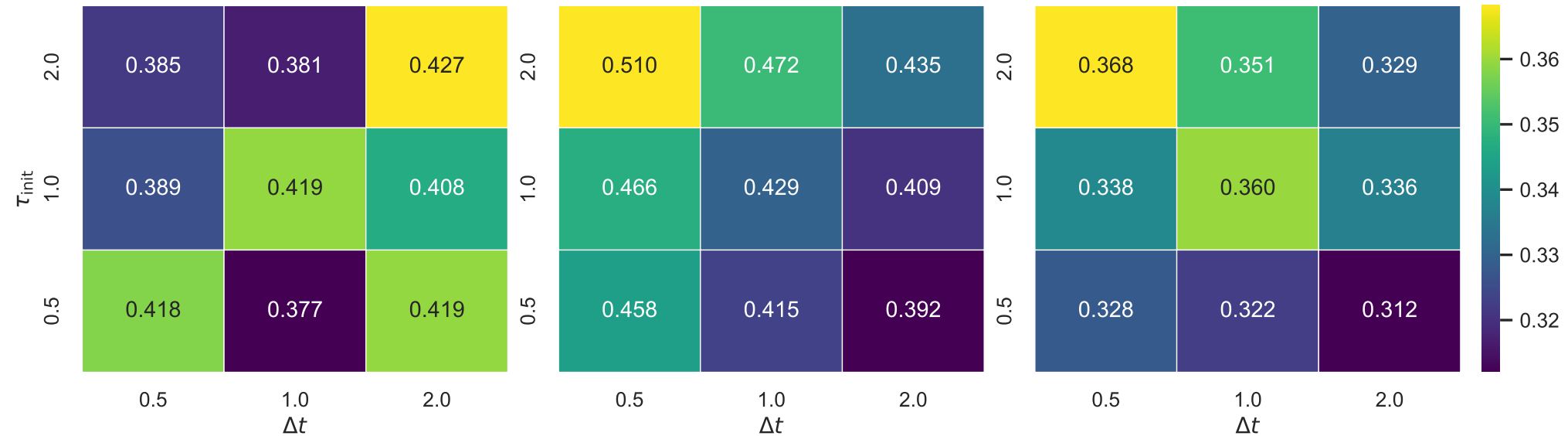
Hybrid-CfC-style
