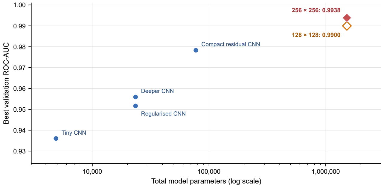
Validation performance versus model size
