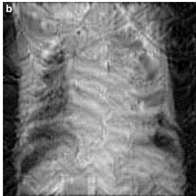
DeepDream (60 steps)
