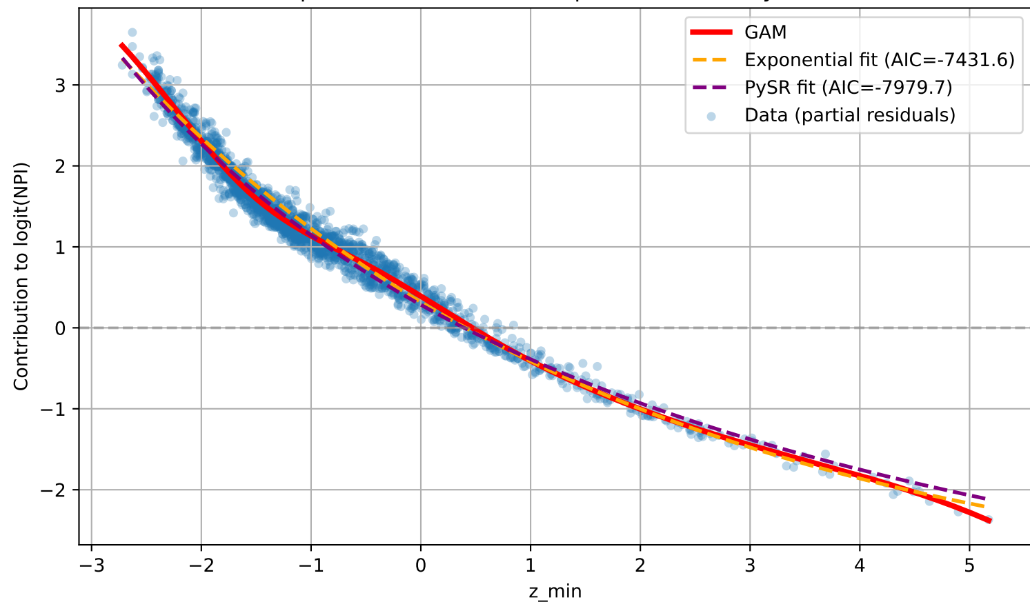
Pupil Min Effect: GAM vs Exponential Fit vs PySR Fit
