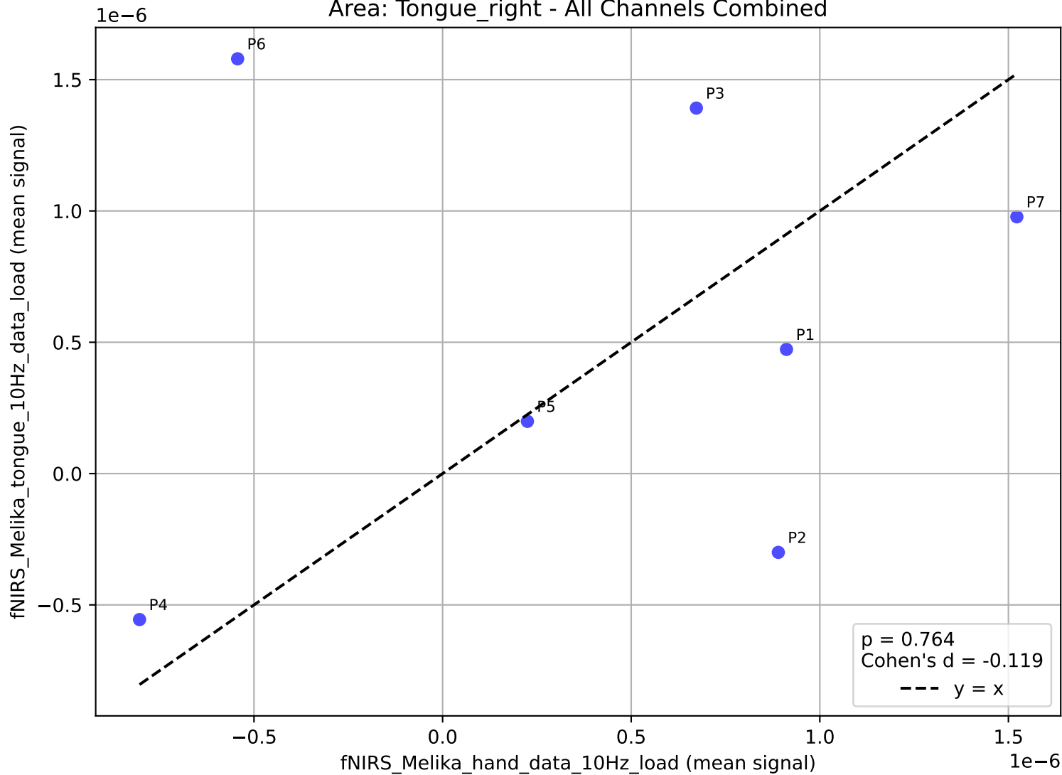
Area: Tongue_right - All Channels Combined
