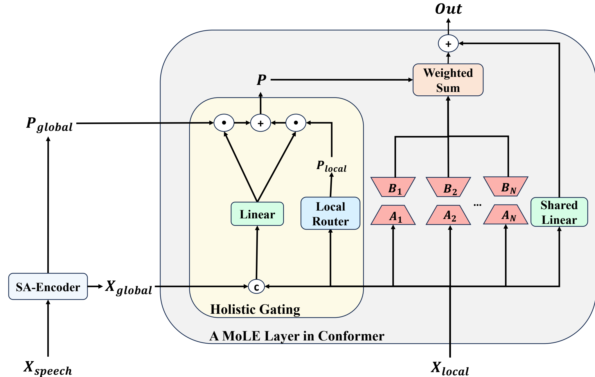
(c) MoLE with Holistic Gating used in H-SAGE
