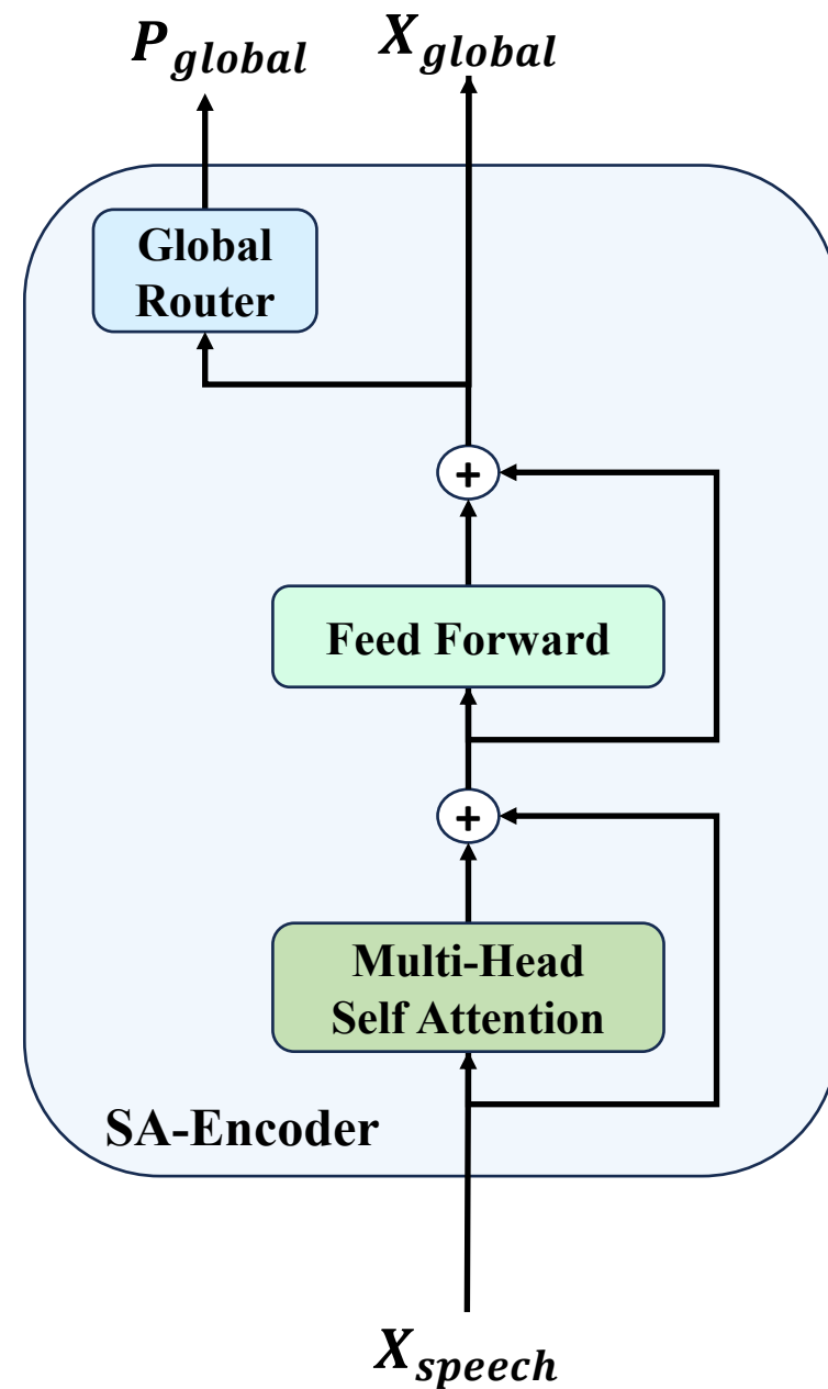
(b) Structure of SA-Encoder
