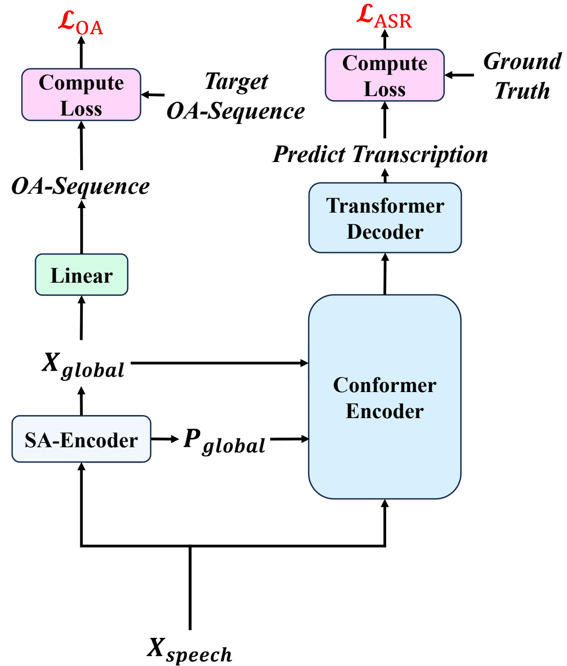
(a) Training of H-SAGE
