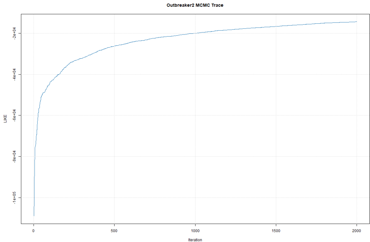
Figure 2. MCMC trace plot — log-posterior probability over iterations. A well-mixed chain shows stable fluctuation around a mean value (no upward/downward drift). If the trace shows a long burn-in slope or multiple plateaux, the chain may not have converged; consider increasing iterations or checking input data quality.
