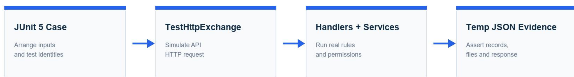
Figure 2. Handler-level unit testing method
