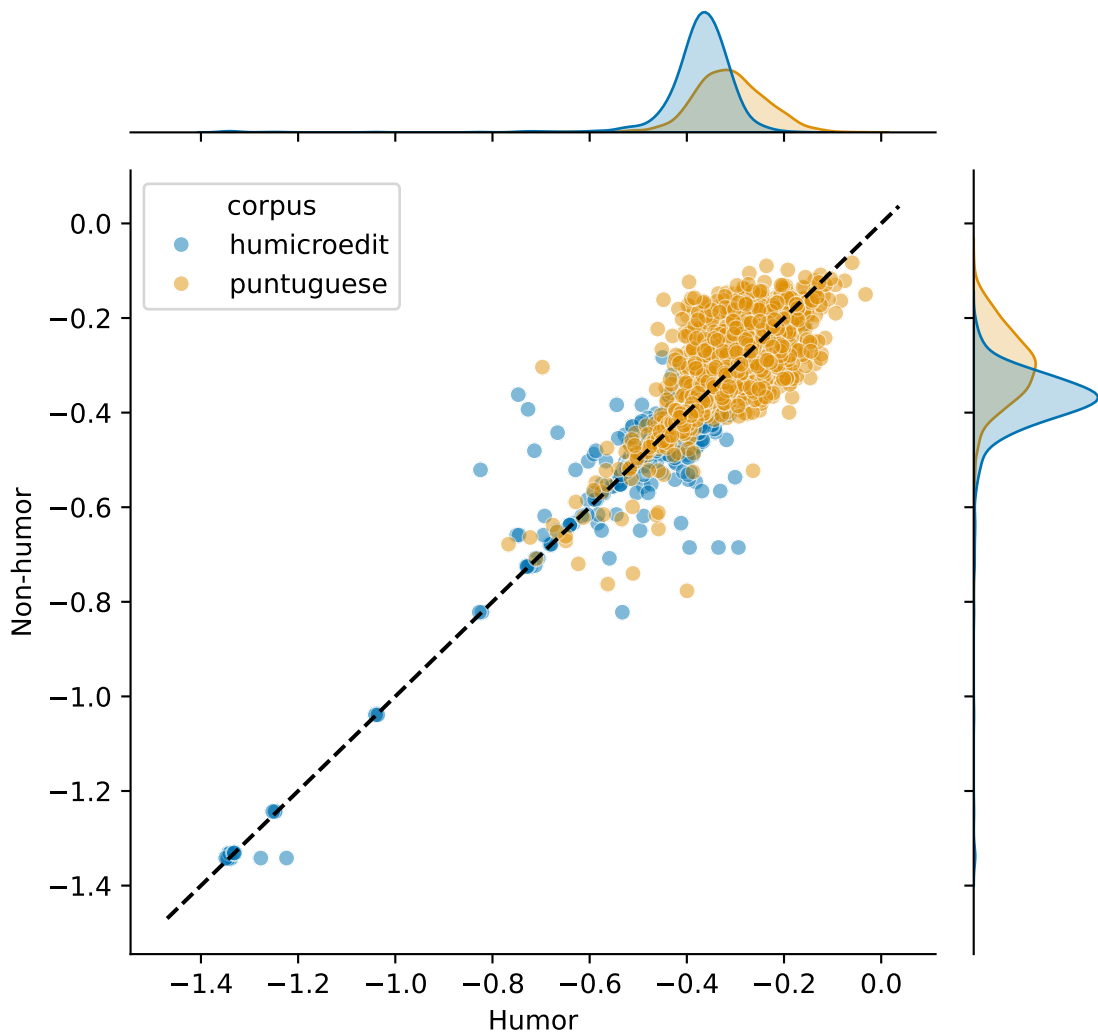
Quantum Incongruity values for humor/non-humor pairs
