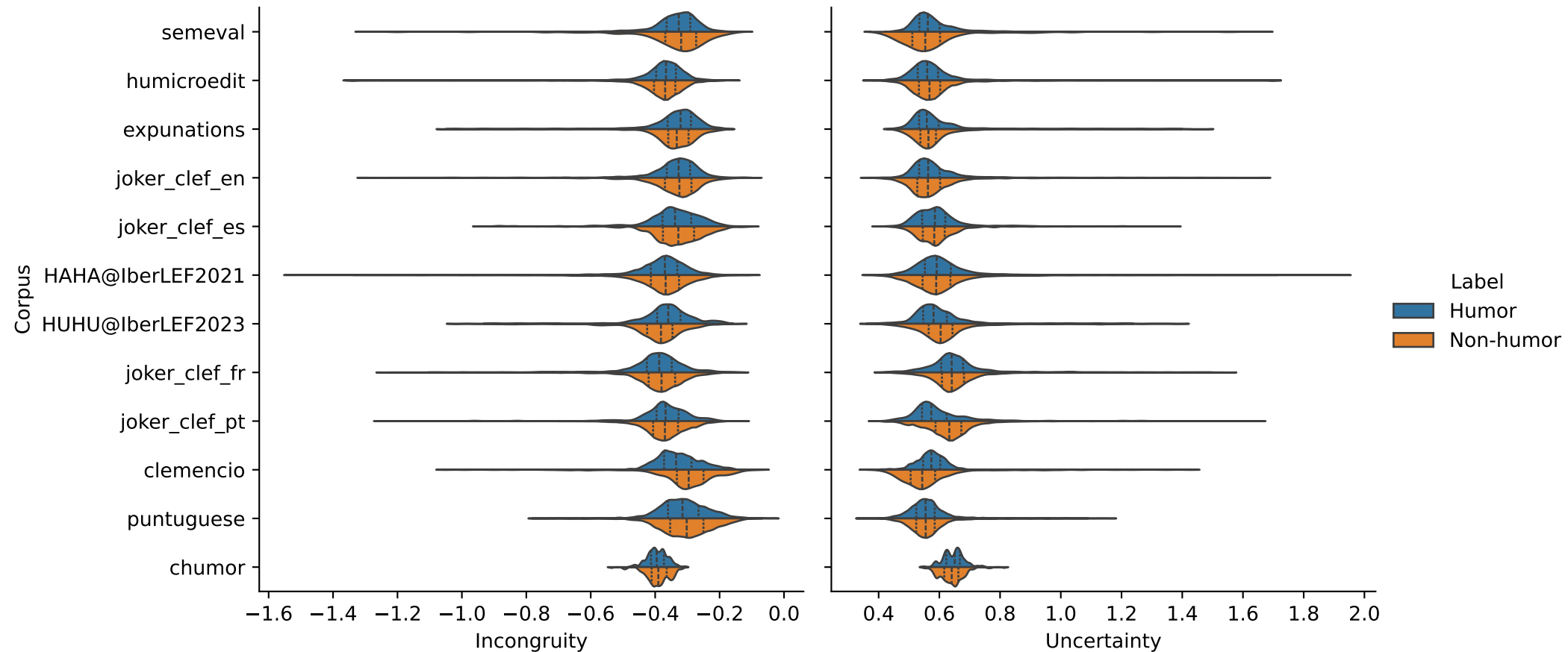
Quantum Entropy metrics using multilingual embeddings
