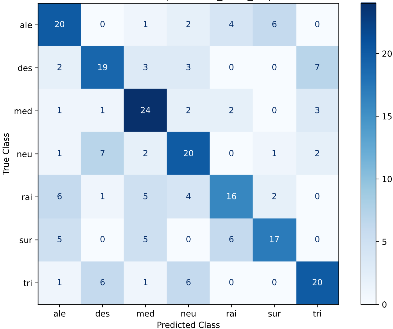
Confusion Matrix - SVC | ComParE_2016_6k | Seed 2025
