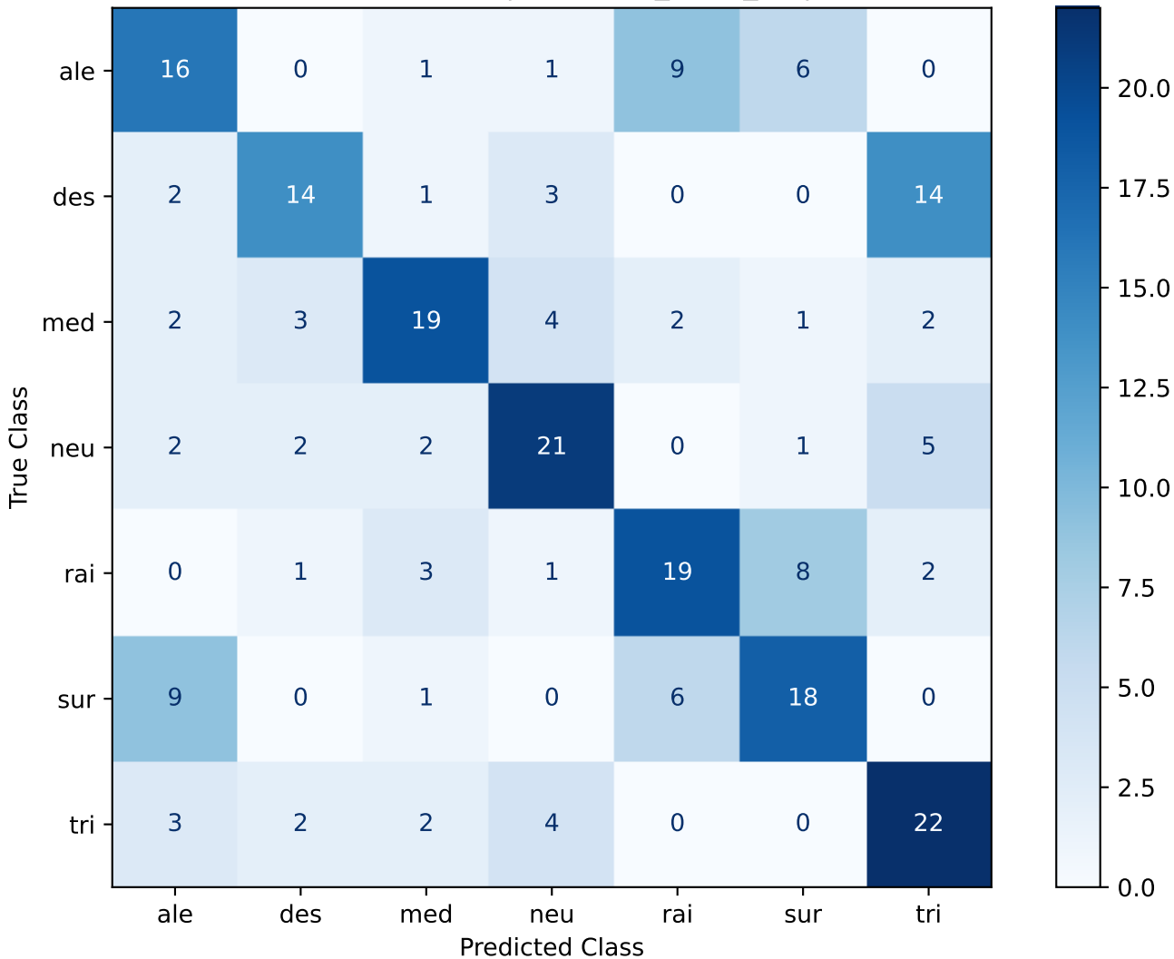
Confusion Matrix - SVC | ComParE_2016_6k | Seed 42
