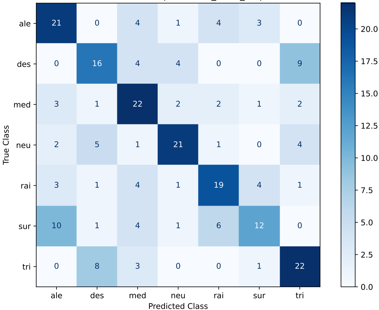
Confusion Matrix - SVC | ComParE_2016_6k | Seed 97
