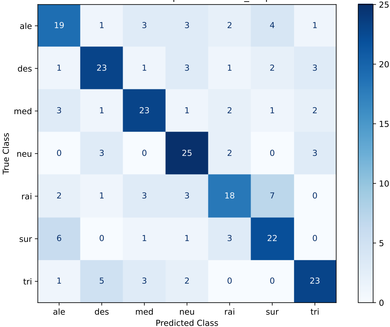
Confusion Matrix - SVC | eGeMAPsv02_88 | Seed 123
