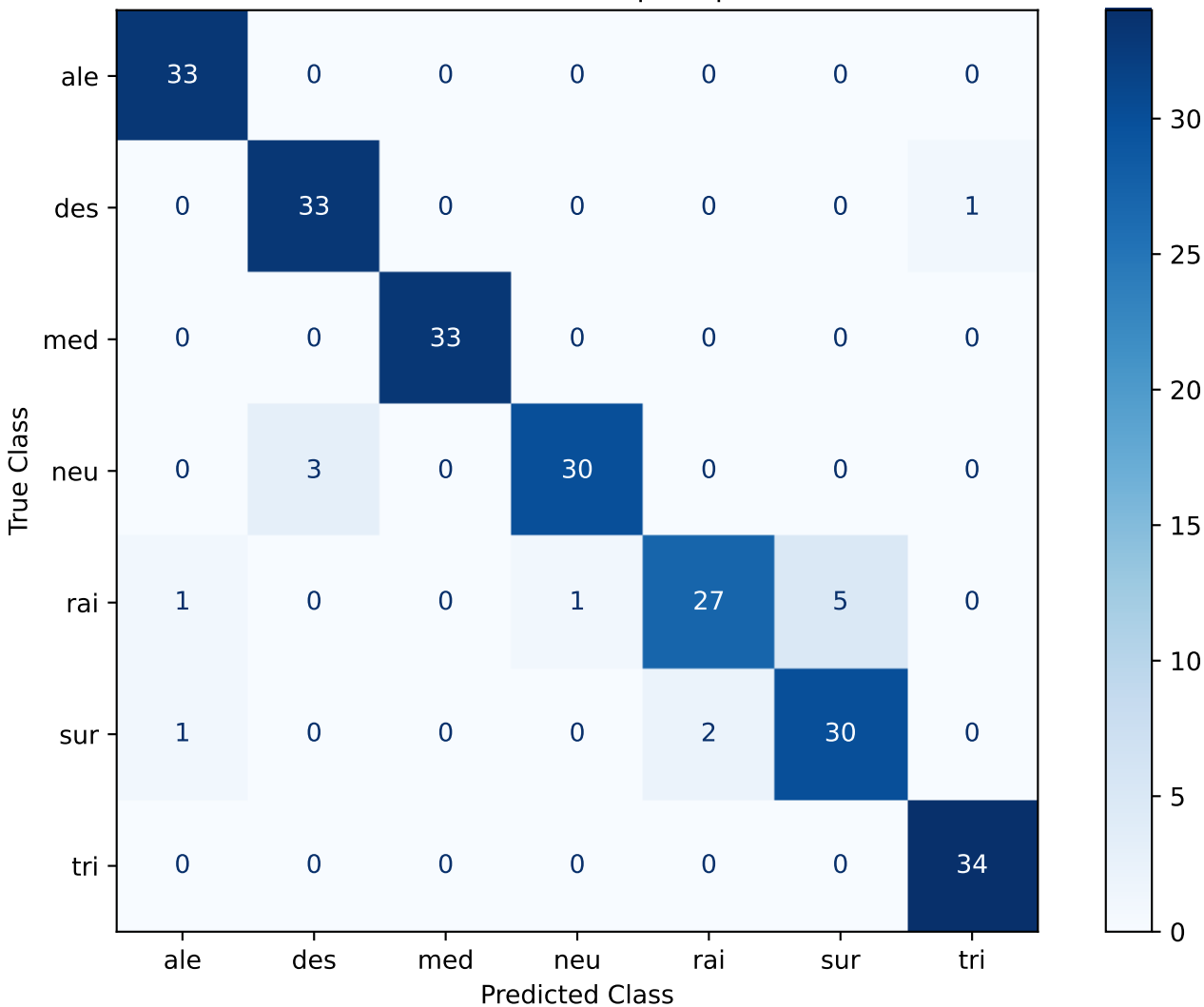
Confusion Matrix - SVC | frill | Seed 123
