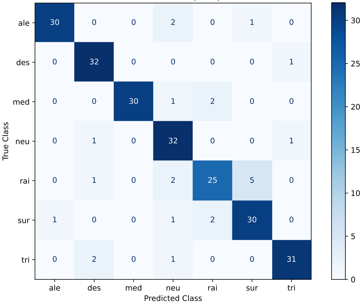
Confusion Matrix - SVC | frill | Seed 97
