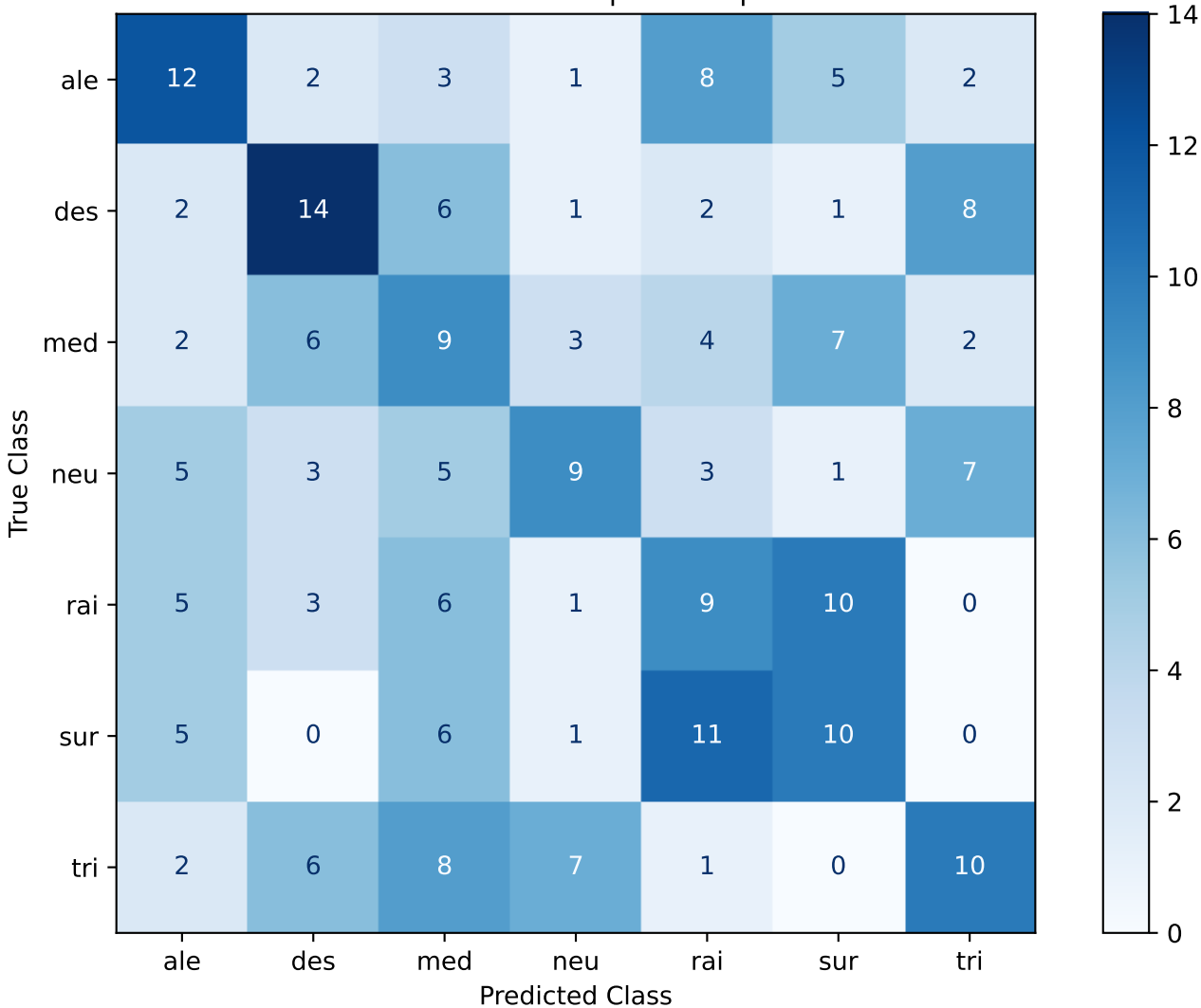
Confusion Matrix - SVC | hubert | Seed 123
