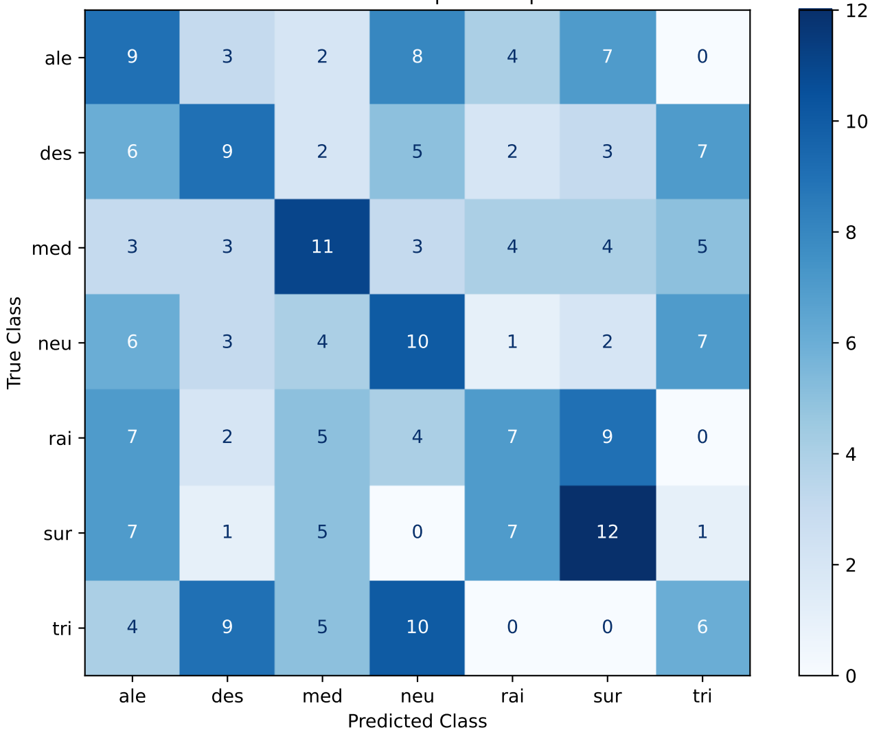
Confusion Matrix - SVC | hubert | Seed 2025
