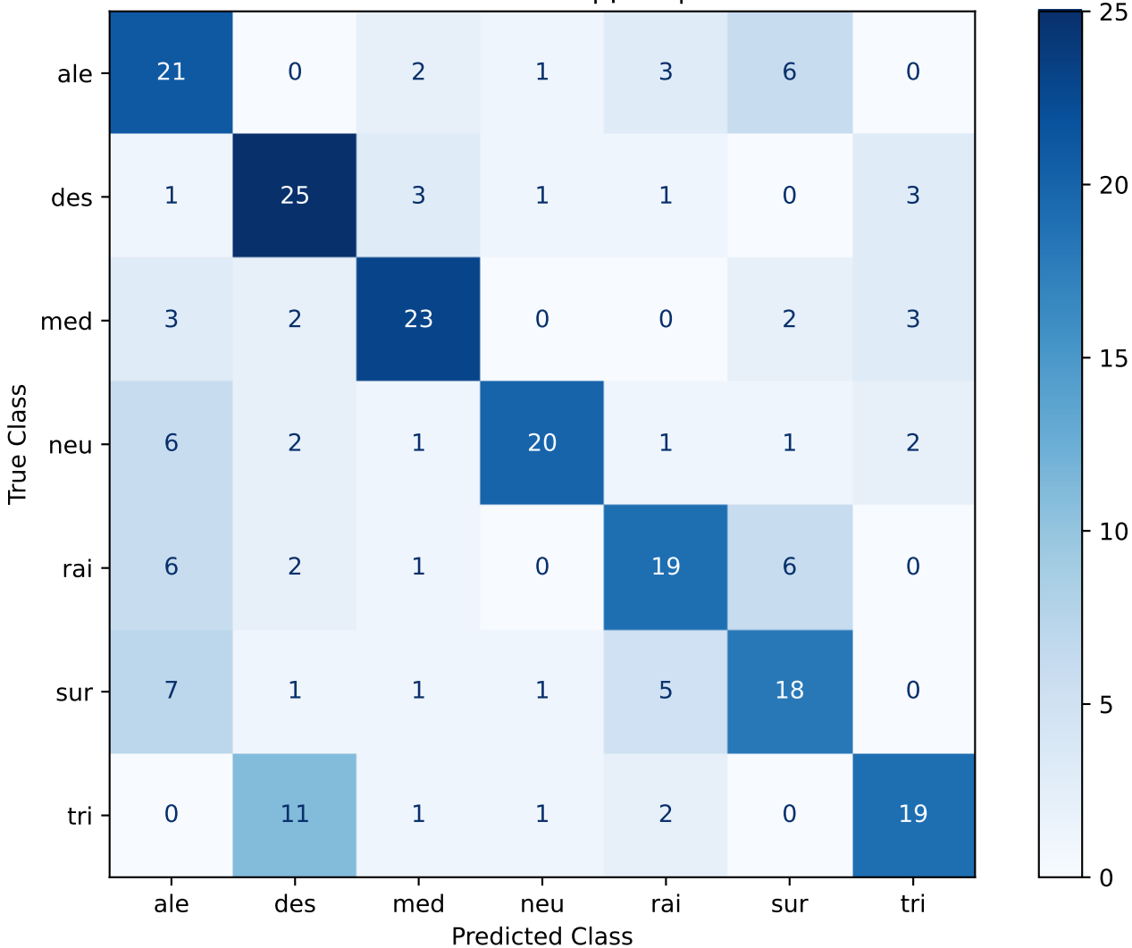
Confusion Matrix - SVC | pAA | Seed 123
