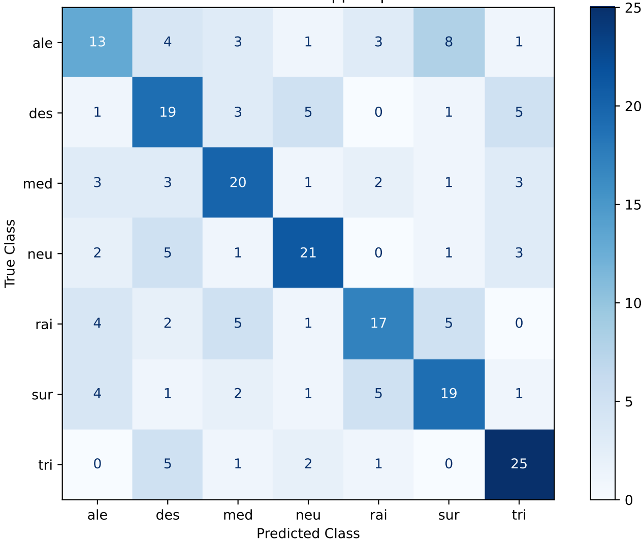
Confusion Matrix - SVC | pAA | Seed 2025
