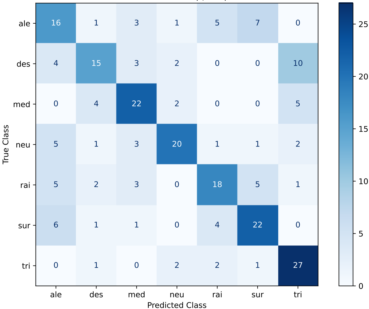
Confusion Matrix - SVC | pAA | Seed 42
